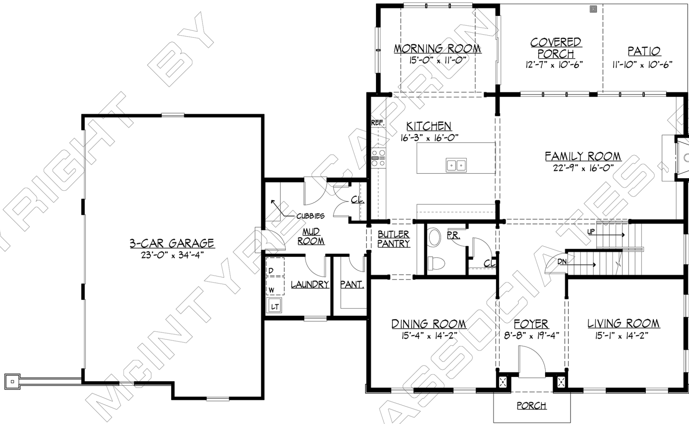
FIRST FLOOR PLAN 2,036 SQ. FT. TOTAL 3,788 SQ. FT.
